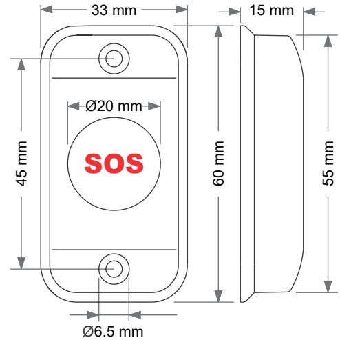
All dimension are in mm tolerance ±0.2mm
