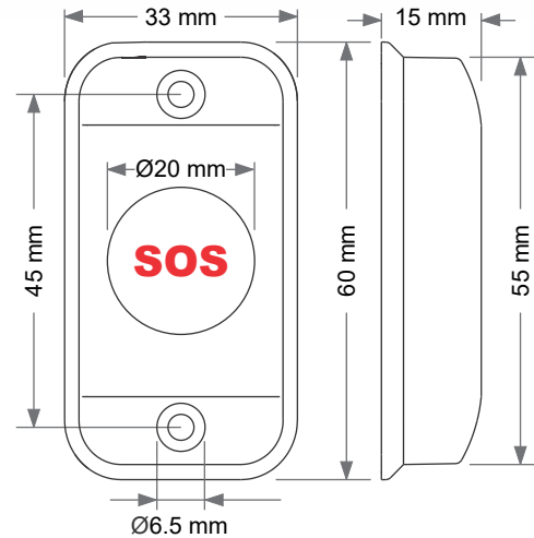
All dimension are in mm tolerance ±0.2mm
