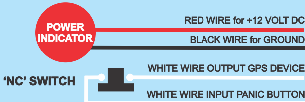
Special Automotive Cable With 4 Numbers 0.5 Sq mm Wire FLYR-B
