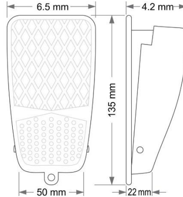
All dimension are in mm tolerance ±0.2mm
