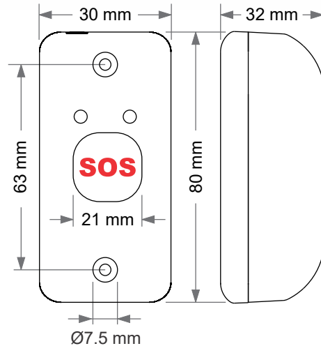
All dimension are in mm tolerance ±0.2mm
