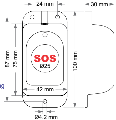
All dimension are in mm tolerance ±0.2mm
