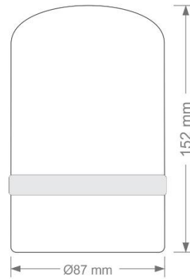
All dimension are in mm tolerance \pm 0.2 mm
