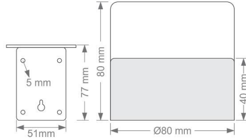
All dimension are in mm tolerance ±0.2mm
