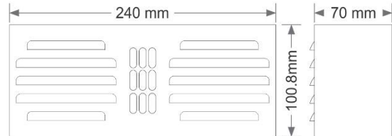
All dimension are in mm tolerance \pm 0.2\text{mm}
