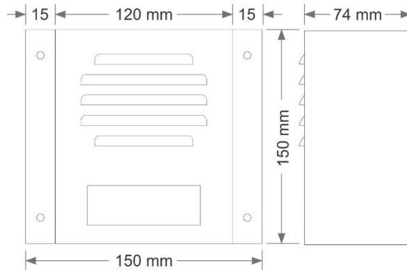
All dimension are in mm tolerance \pm 0.2\text{mm}
