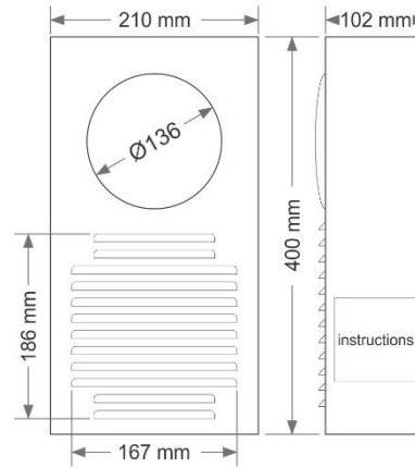
All dimension are in mm tolerance ±0.2mm
